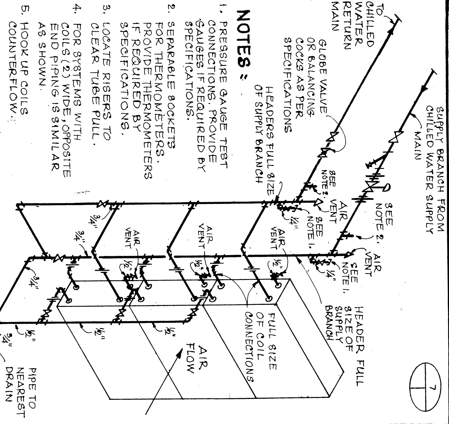
MULTIPLE HIGH VERTICAL WATER COIL PIPING (THROTTLING CONTROL VALVE)
